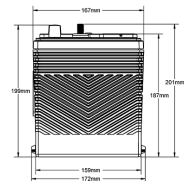
ODP-AGM34M LEFT POSITIVE DUAL TERMINALS (SAE & STUD)
