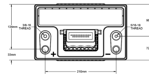
ODP-AGM34M LEFT POSITIVE DUAL TERMINALS (SAE & STUD)
