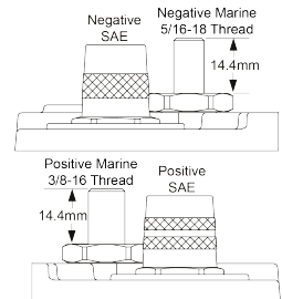
ODP-AGM34M LEFT POSITIVE DUAL TERMINALS (SAE & STUD)
