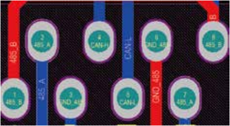
Puerto RS485/CAN
