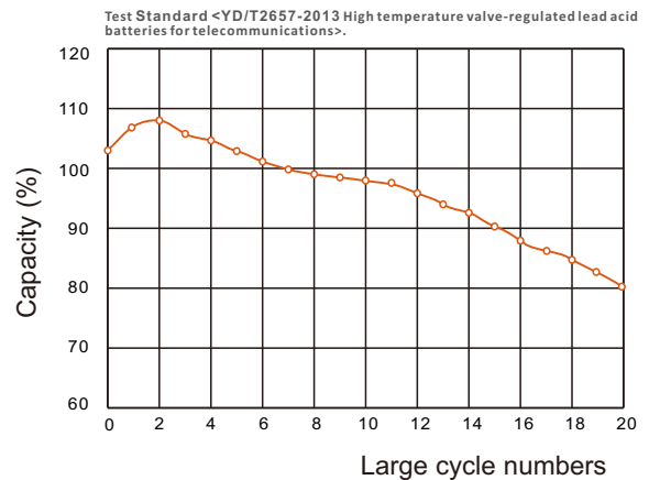
High temperature deep cycle life @ 55°C
